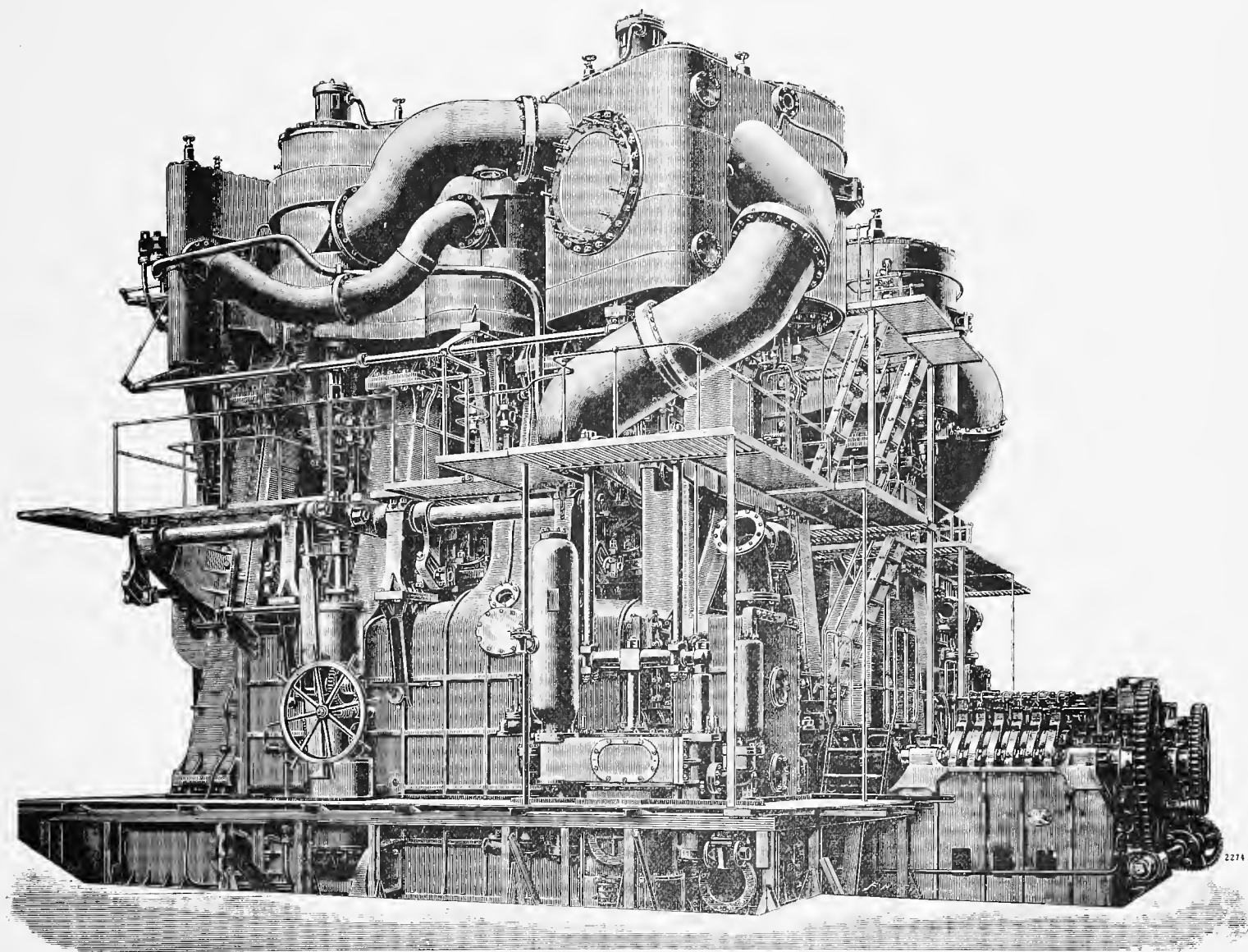
GENERAL VIEW OF THE QUADRUPLE-EXPANSION ENGINES OF THE INTERNATIONAL NAVIGATION CO.'S TWIN-SCREW STEAMSHIP KENSINGTON.
